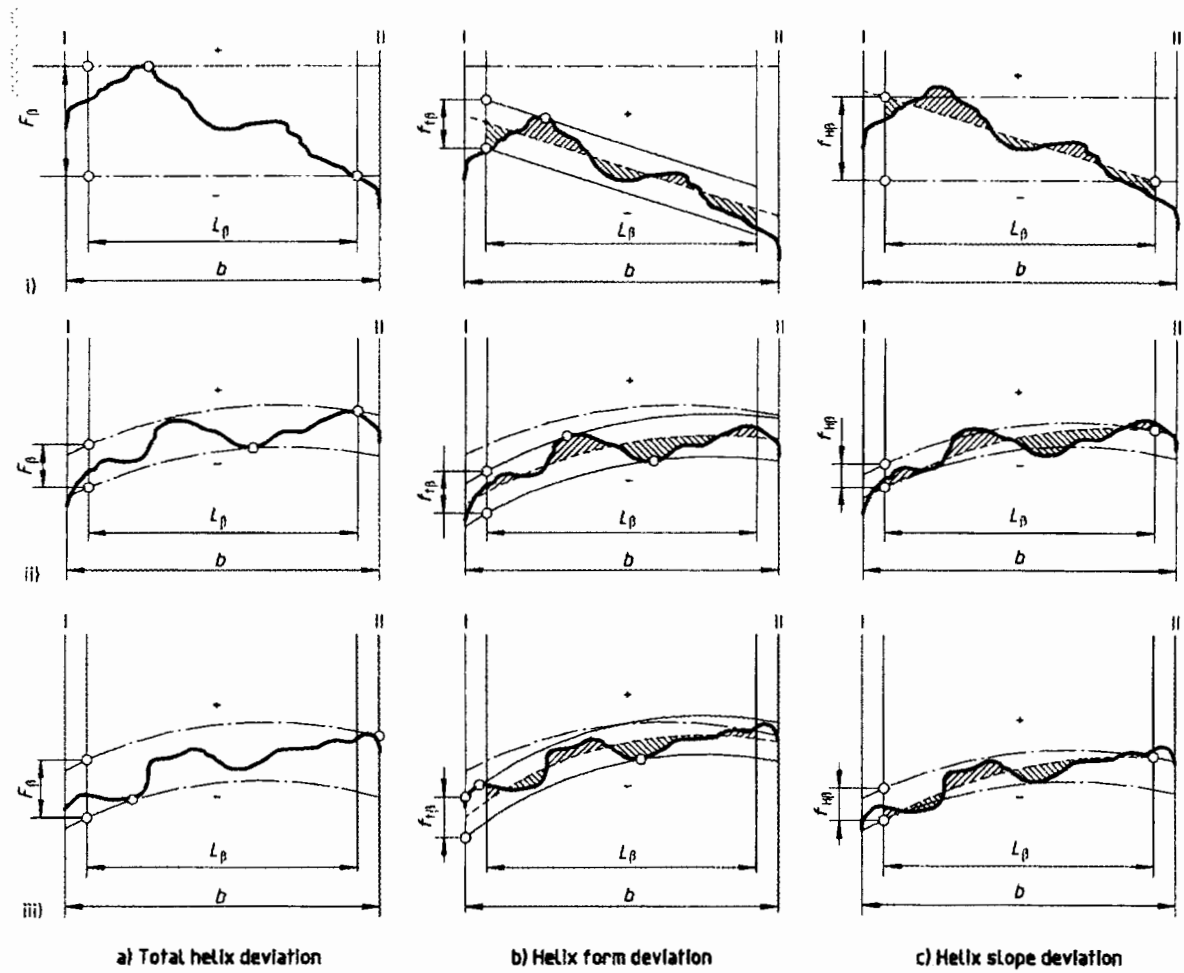
Figure 3 — Helix deviations
