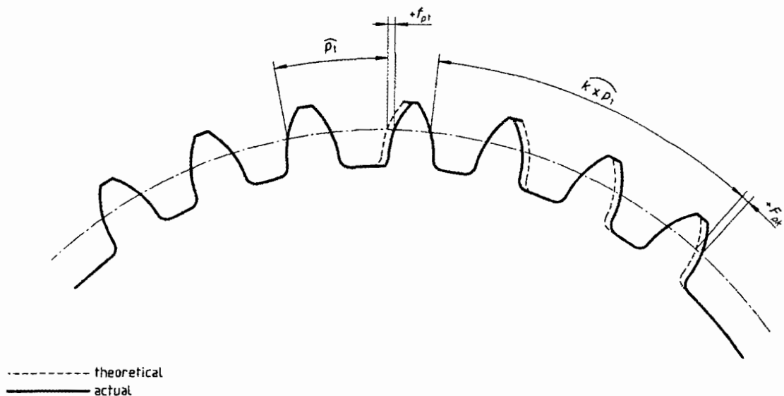
Figure 1 — Pitch deviations
