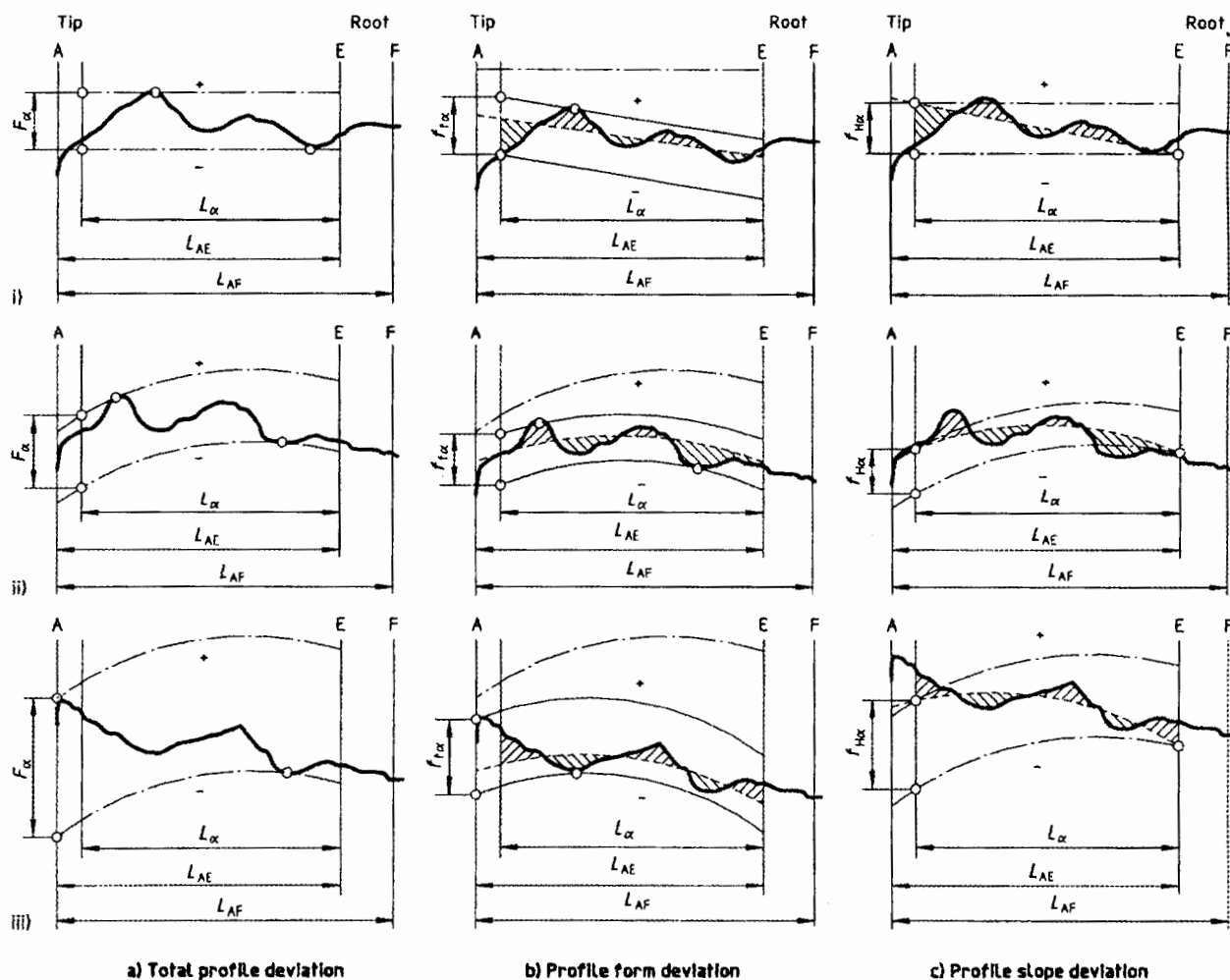
Figure 2 — Profile deviations
